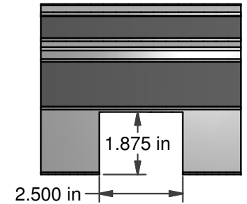
FRONT BUMPER TRIM DIAGRAM
