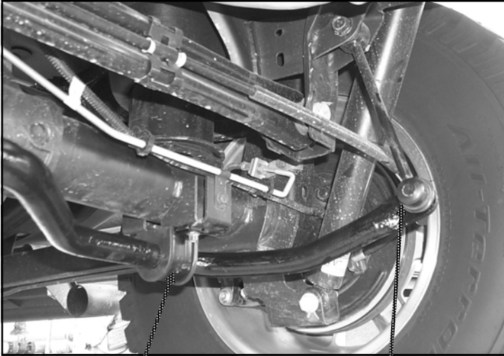
D-Shaped Poly-Bushing and U-Plate
